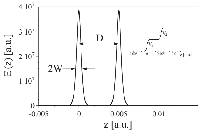
FIG. 1. The two electric fields E(z) = (E_1/2)\text{sech}^2(z/W) + (E_2/2)\text{sech}^2[(z-D)/W] and their associated potential V(z) = -\int_{-\infty}^z dz' E(z') . We have graphed the field and the potential for the parameters used in the simulations discussed below, D = 0.005 a.u. and W = 0.05/c .
