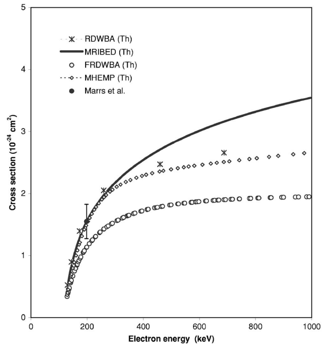
FIG. 10. Same as Fig. 6 for \text{U}^{91+} with the experimental data of [48] as solid circles, the RDWBA results of [32] as the dotted curve with asterisks, and FRDWBA predictions of [36] as open circles.
